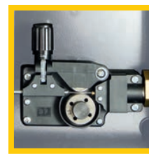
MIGA 380: Trainafilo 2 rulli D.30mm 2 rolls wire feeder D.30mm
