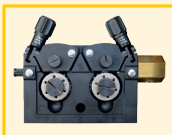
Trainafilo 4 rulli D.37mm 4 rolls wire feeder D.37mm
