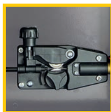
MIGA 320: Trainafilo 2 rulli D.25mm 2 rolls wire feeder D.25mm
